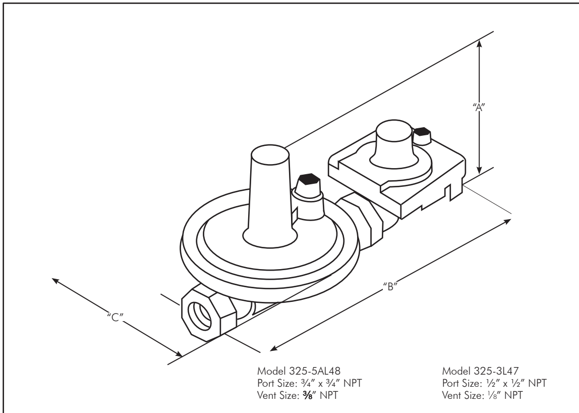
FIG. 4-36B Maxitrol 325 Pressure Regulator O.A.R.A. Type 90/95 Pressure Regulator
